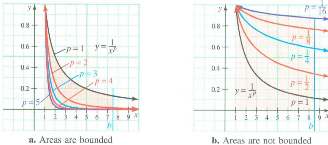
Figure 8.15 Graphs for the p -series test
