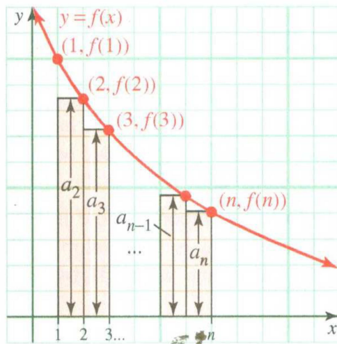
a. The k th rectangle has height f(k+1) = a_{k+1}
