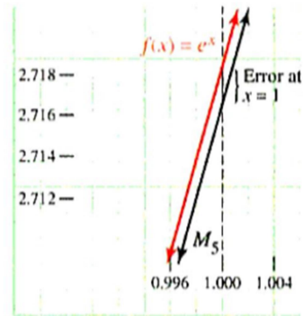
b. Zoom showing the error at x = 1
