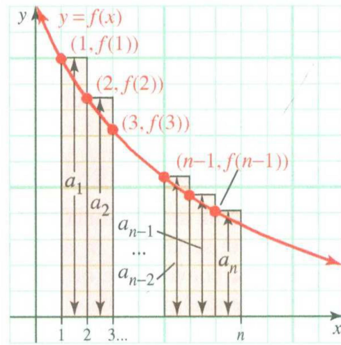
b. The k th rectangle has height f(k) = a_k
